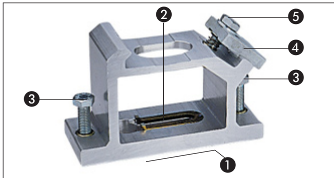
Rail support for regular cutting
