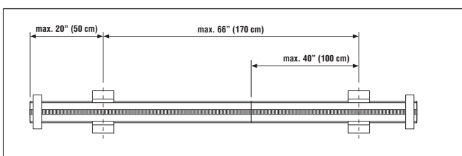
Maximal permissible rail support distance
