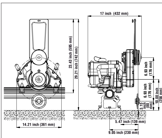
Main dimensions of the DS TS20-E (in inch / mm)
